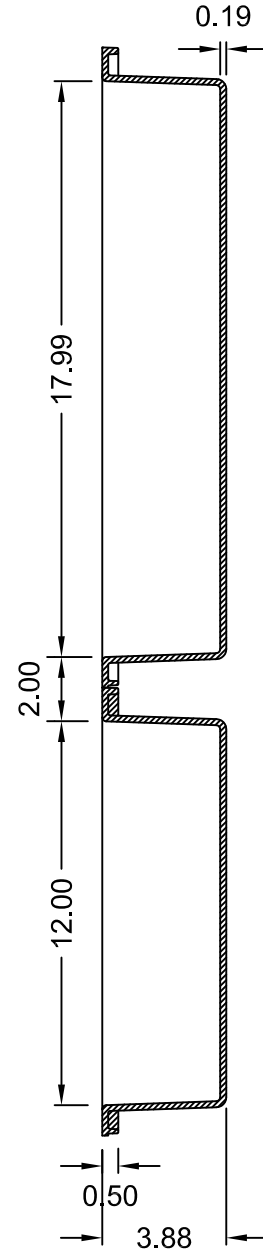
SECTION B-B
