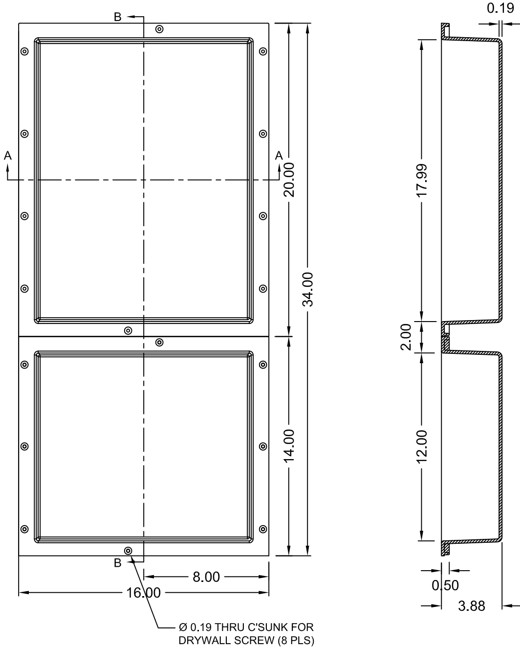
SECTION B-B
